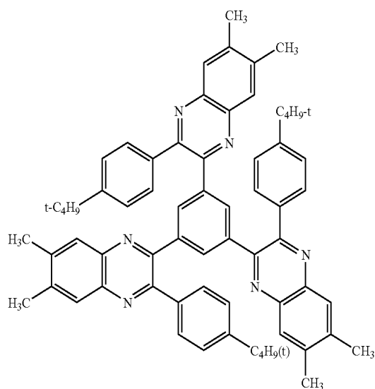
Compound described in Macromolecules 31, 6434 (1989)
