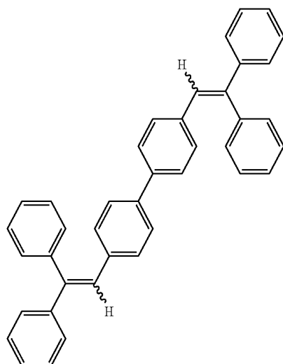
Compound described in Appl. Phys. Lett. 67, 3853 (1995)
