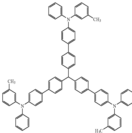
Compound described in JP-A 10-312073
