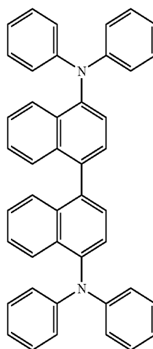
Compound described in 11-152253
